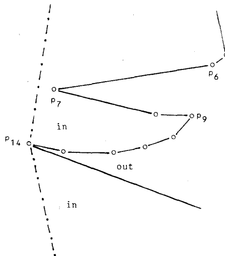
FIG. 15. “Conceptual edges” for outer triangulation.
