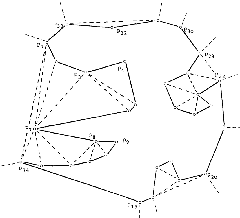
FIG. 14. Outer triangulation of a simple 33-gon.
