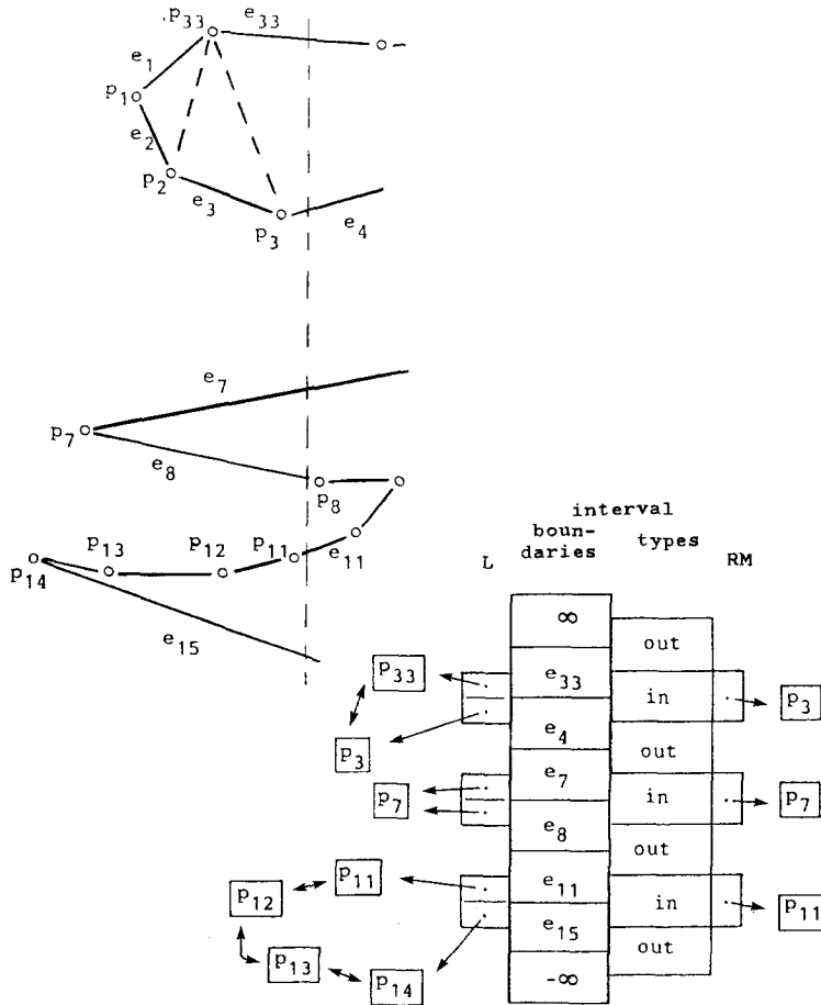
FIG. 6. Structure Y-C in a typical situation.
