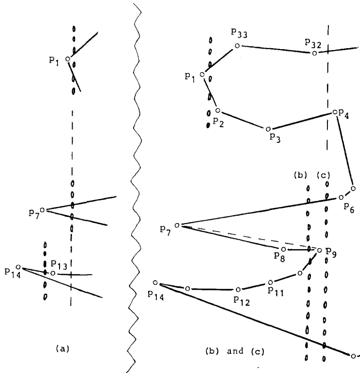
FIG. 13. Possible situations in sample polygon: the dashed line is the global sweep line; heavily dashed lines represent local sweep lines.
