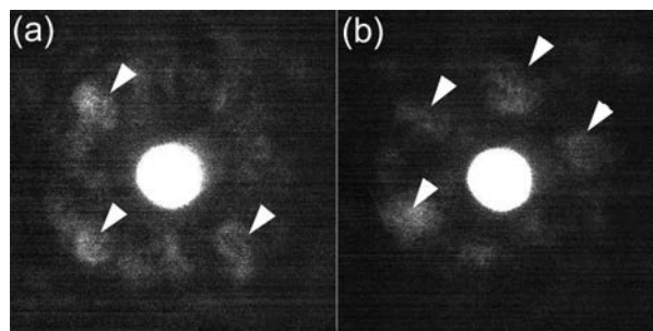
Figure 3: Scanning NBED patterns including weak diffraction spots. Probe size is \sim 0.5 nm with beam convergence semi-angle of \sim 3 mrad. Beam incidence \sim [001]_{\text{bcc-Fe}} (a) and \sim [111]_{\text{bcc-Fe}} (b). Arrowheads indicate 110 reflections of bcc-Fe.
