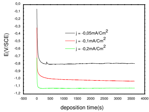
Fig. 4. Variation of potential vs. time during cathodic deposition at j = -0.05, -0.1 and -0.2 \text{ mA cm}^{-2}
