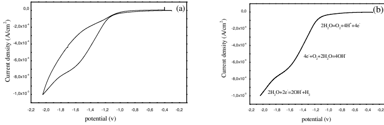
Fig. 2. Cyclic voltammetry curves obtained with TA6V substrates in \text{Ce}(\text{NO}_3)_3 , 6\text{H}_2\text{O} and mixed water-ethyl alcohol solutions at 0.01 \text{ mol.L}^{-1} , ( 10 \text{ mV/s} ).
