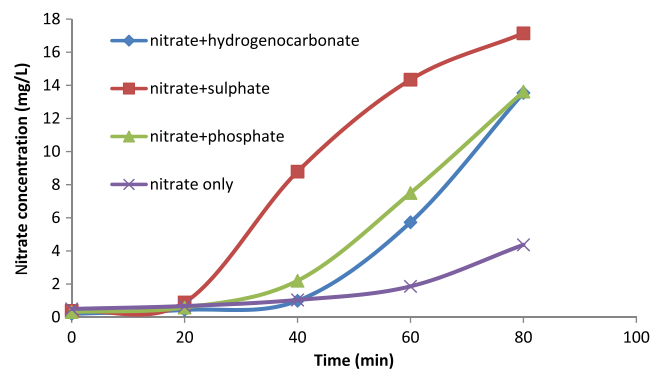
Figure 6 Time dependence of transport of nitrate in contact with different accompanying anions for the RPA membrane (receiver phase: 0.1 \text{ M NaCl} ).
