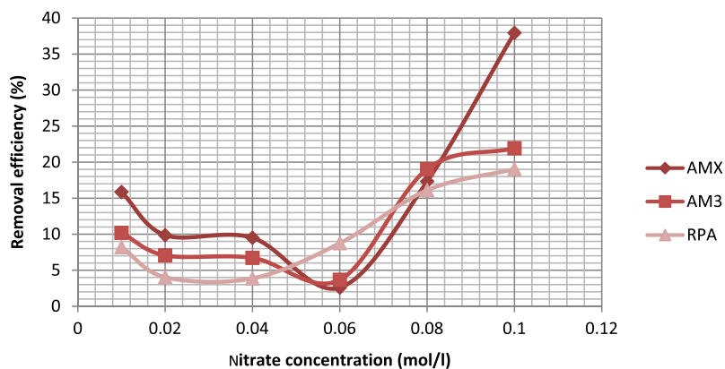
Figure 8 Contribution of the membrane structure on the nitrate transport in the range 0.01 M to 0.1 M of nitrate for AMX AM3 and RPA anion-exchange membranes.
