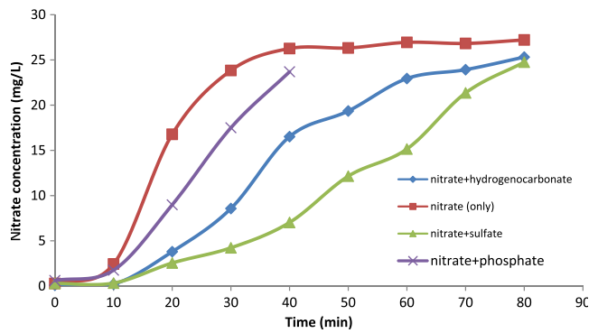
Figure 4 Time dependence of transport of nitrate in contact with different accompanying anions for the AMX membrane (receiver phase: 0.1 \text{ M NaCl} ).
