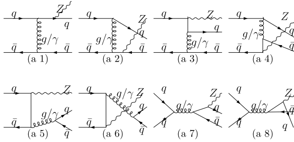
Fig. 4. Tree-level diagrams contributing to the partonic subprocess q + \bar{q} \rightarrow Z + q + \bar{q} at \mathcal{O}(\alpha_s^2) (with a virtual gluon). Interferences of diagrams (a 5)–(a 8) with a virtual photon or Z boson (gluon) with diagrams (a 1)–(a 4) with a virtual gluon (photon or Z boson) contribute at \mathcal{O}(\alpha^2\alpha_s) .
