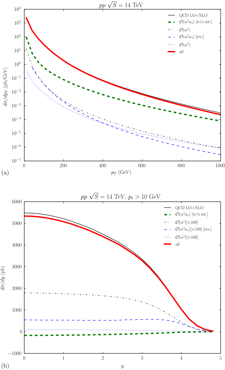
Fig. 10. Same as in Fig. 8, but for pp \rightarrow Z + X at \sqrt{S} = 14 \text{ TeV} (LHC).
