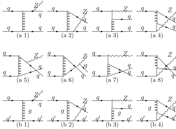
Fig. 6. Tree-level diagrams contributing to the partonic subprocesses q + q \rightarrow Z + q + q and q + q' \rightarrow Z + q + q' at \mathcal{O}(\alpha_s^2) . Interferences of diagrams (a 5)–(a 8) with the gluon replaced by a photon or Z boson with diagrams (a 1)–(a 4) contribute at \mathcal{O}(\alpha^2\alpha_s) .
