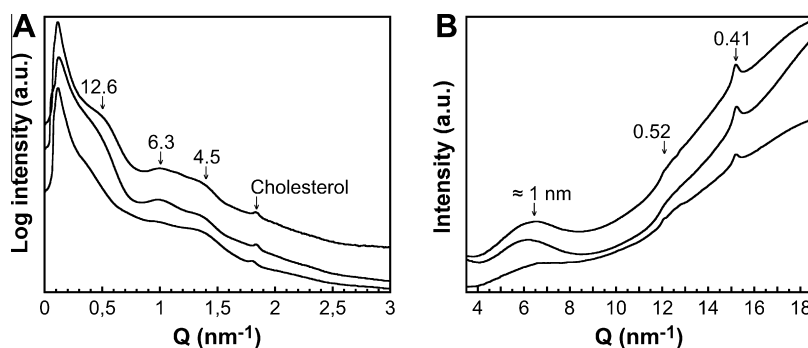
Fig. 2. X-ray diffraction data obtained at 32 °C of SC pretreated at 32 °C for 24 h in neat PBS solution (middle curve), 20 wt% glycerol in PBS (top curve), or 20 wt% urea in PBS (bottom curve). (A) SAXD data. (B) WAXD data. The numbers by the arrows give the d -spacing in nm. One replicate per SC sample was measured.
