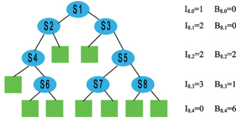
Fig. 1. A digital search tree built on eight strings s_1, \dots, s_8 (i.e., s_1 = 0\dots, s_2 = 1\dots, s_3 = 01\dots, s_4 = 11\dots , etc.) with internal (ovals) and external (squares) nodes, and its profiles.
