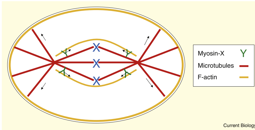
Figure 2. Model by Woolner et al. [9] for myosin-X's involvement in spindle-length regulation. Interaction of astral microtubules and cortical F-actin stretch the spindle while microtubule-bound myosin-X pulls on spindle-associated F-actin thereby shortening it.
