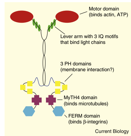
Figure 1. Model of the domain structures of myosin-X and their functional associations [10].
