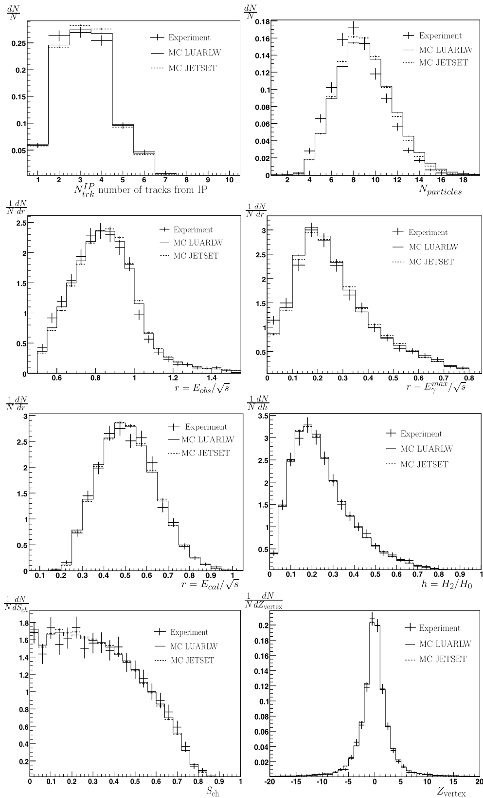
Fig. 2. Properties of hadronic events produced in uds continuum at 3.12 GeV. Here N is the number of events, S_{ch} is sphericity, H_2 and H_0 are Fox-Wolfram moments. Integrals of all distributions are normalized to unity.
