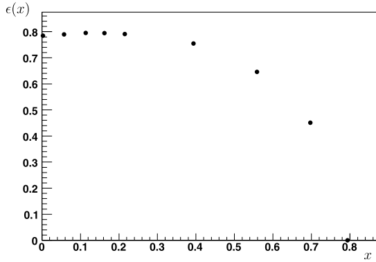
Fig. 3. Hadronic detection efficiency versus variable x of Eq. (3) at 3.52 GeV in the first scan.
