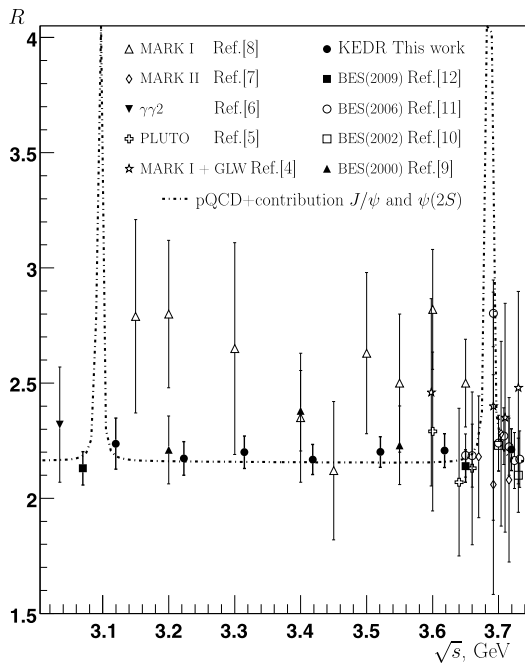
Fig. 4. The quantity R versus the c.m. energy and the sum of the prediction of perturbative QCD and a contribution of narrow resonances.
