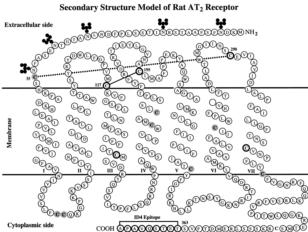
Fig. 1. A secondary structure model of the rat AT 2 receptor. The location of 14 cysteine residues is indicated in the proposed membrane topology. Five cysteines conserved between AT 1 and AT 2 receptors are shown in circles and the proposed disulfide interactions in the extracellular domain are indicated. Potential glycosylation sites and the octapeptide-epitope tag used in the immunoblotting experiments are shown.
