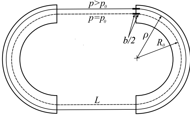
Fig. 1. The storage ring.
