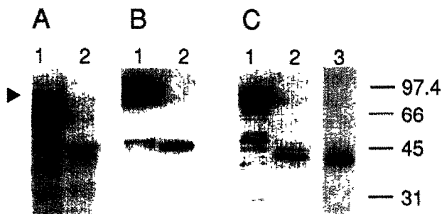
Fig. 3. SDS-PAGE/immunoblot analysis of the fusion protein. (A) Stained with Coomassie brilliant blue. (B) Immunoblot with an anti-MBP antibody. (C) Immunoblot with an anti-H6H antibody mAb5. Lanes 1 and 2, proteins before and after cleavage with factor Xa, respectively. Lane 3 of C, H6H purified from cultured roots of H. niger . The arrow points to the fusion protein between MBP and H6H. Molecular weights of the standard proteins are indicated on the right in kDa.
