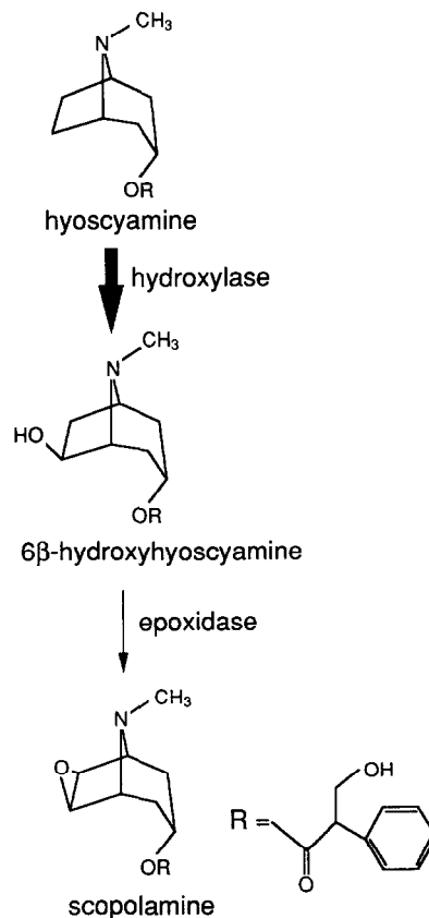
Fig. 1. Conversion of hyoscyamine to scopolamine by way of 6 \beta -hydroxyhyoscyamine. The present study demonstrates that hyoscyamine 6 \beta -hydroxylase catalyzes both the first hydroxylation reaction and the second epoxidation reaction.
