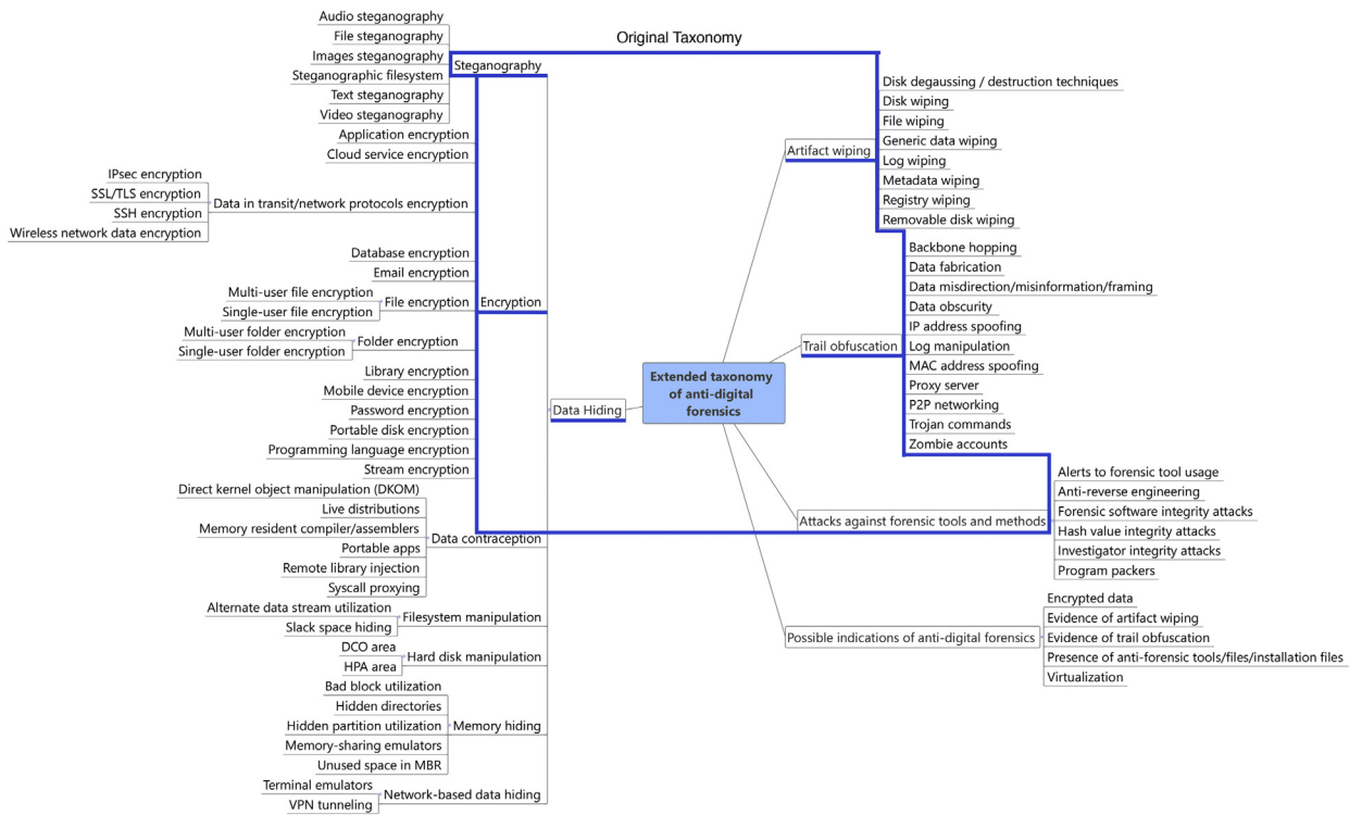
Fig. 1. Extended taxonomy.
