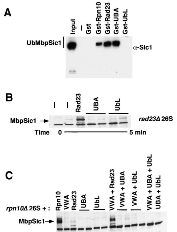
Figure 3. Complementation of rad23Δ Proteasomes Requires Both the Ub Binding UBA Domains and the Proteasome Binding UbL Domain of Rad23
