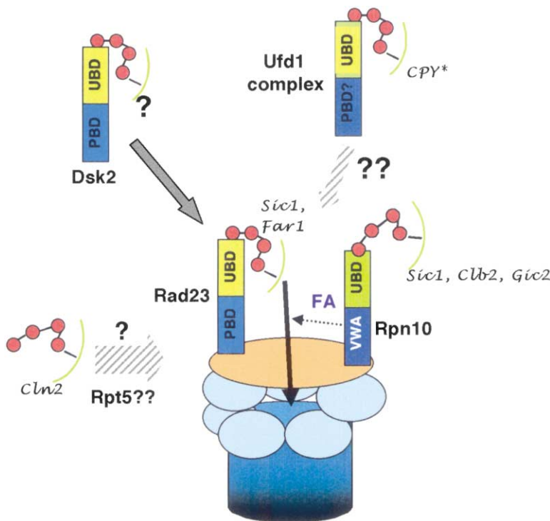
Figure 7. Hypothetical Model for Physiological Targeting Pathways that Deliver Ubiquitinated Substrates to the 26S Proteasome
