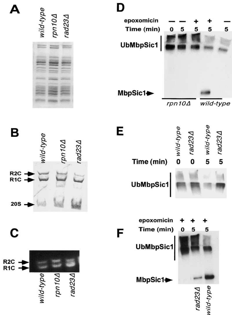
Figure 1. Structural and Functional Characterization of 26S Proteasomes Isolated from rpn10Δ and rad23Δ Mutants by Affinity Chromatography
