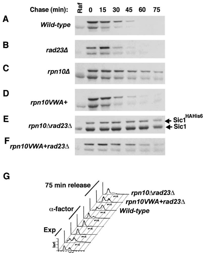
Figure 5. Rpn10 UIM Domain and Rad23 Serve Redundant Roles in Sic1 Turnover In Vivo
