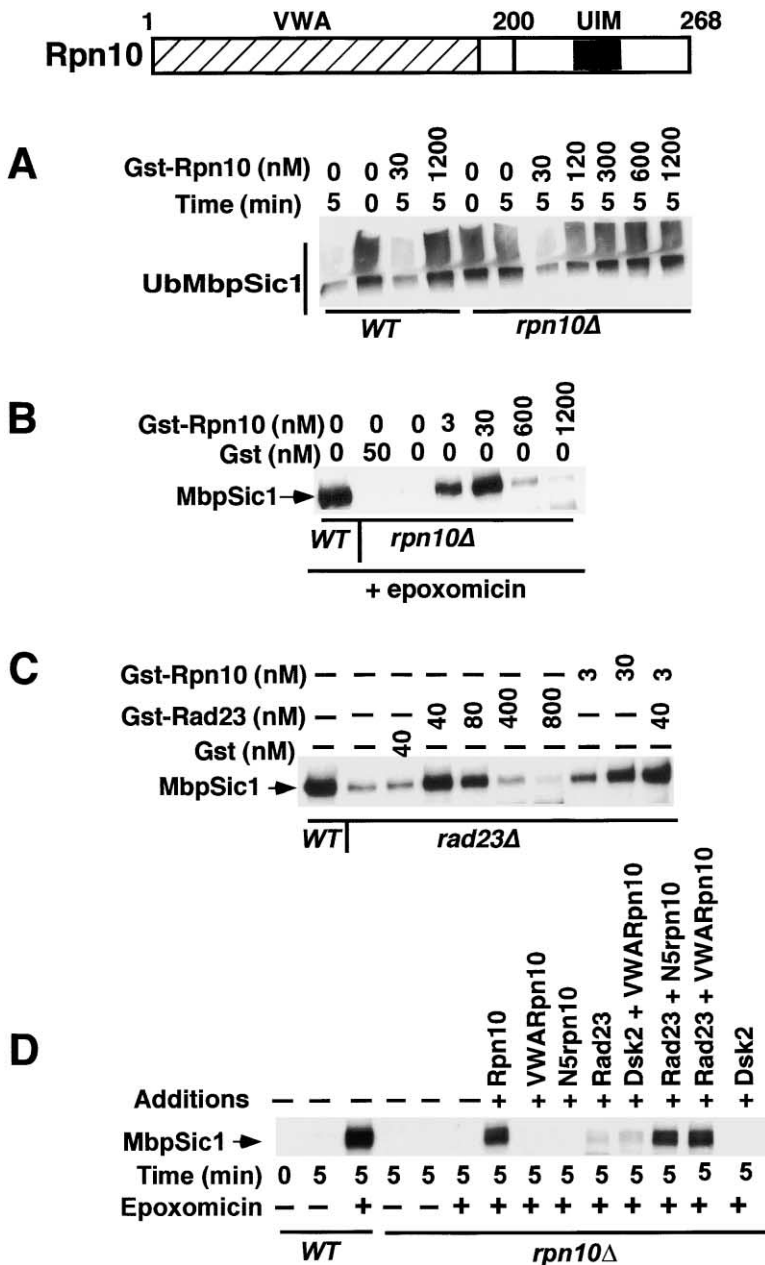
Figure 2. The Degradation and Deubiquitination Defects of rpn10Δ and rad23Δ 26S Proteasomes Can Be Rescued by Recombinant Proteins
