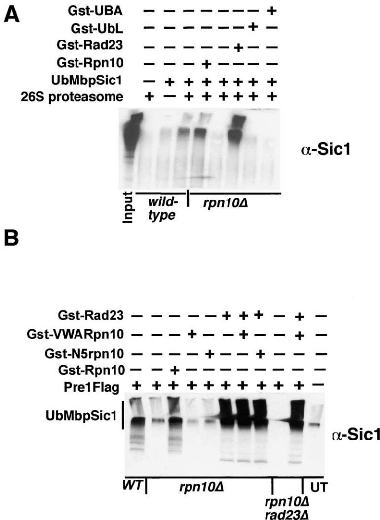
Figure 4. 26S Proteasomes from rpn10Δ Are Defective in Binding UbMbpSic1
