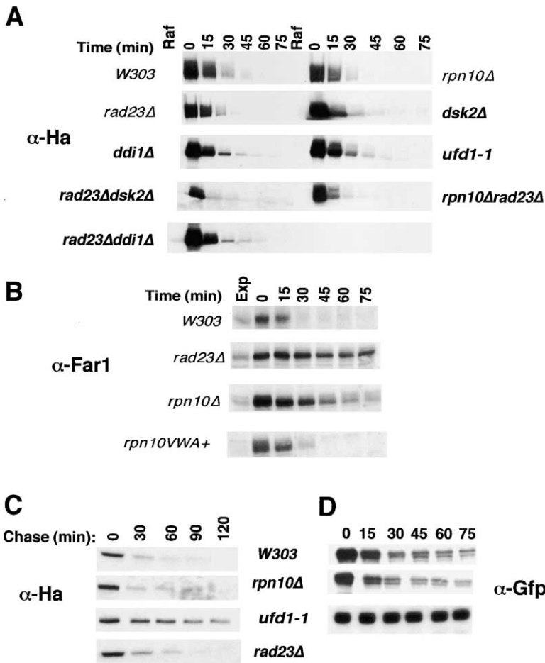
Figure 6. UPS Substrates Have Differential Requirements for Multiubiquitin Chain Receptors In Vivo
