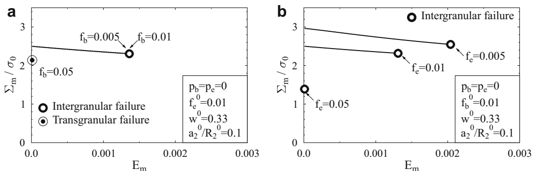
Fig. 9. Influence of the two porosities f_b and f_e on the overall stress–strain response of a doubly voided material.
