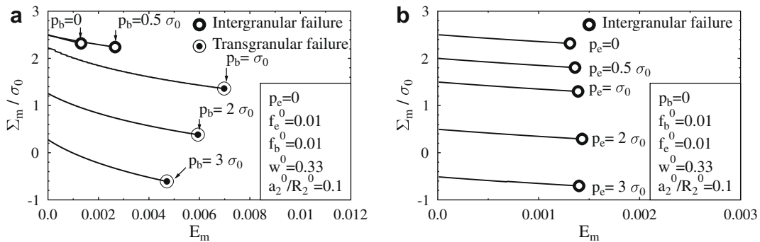
Fig. 8. Influence of the internal pressures p_b and p_e on the overall stress–strain response of a doubly voided material.
