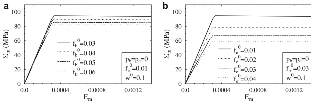
Fig. 2. Influence of the initial porosities f_b^0 and f_e^0 on the overall stress–strain response of a doubly voided material. Initial aspect ratio of the ellipsoidal cavities w^0 = 0.1 . Drained case p_e = p_b = 0 . (a) Influence of the intragranular porosity f_b^0 (spherical voids). (b) Influence of the intergranular porosity f_e^0 (ellipsoidal voids).
