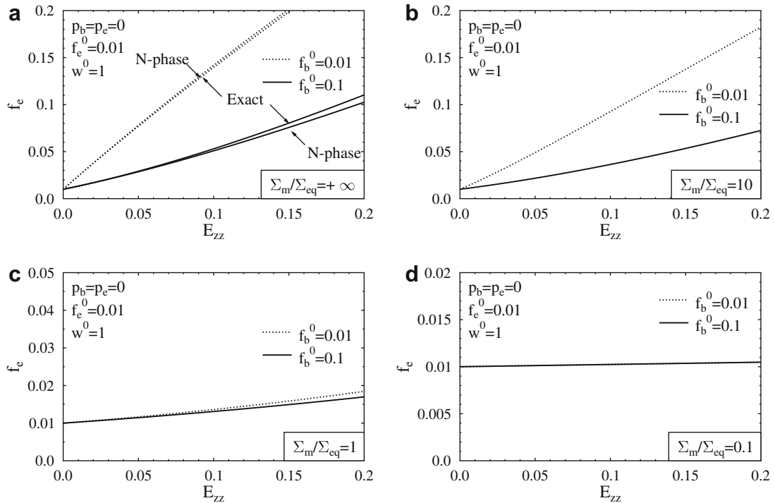
Fig. 5. Influence of the presence of a secondary population of voids (small voids) on the growth of the first population (large voids). Influence of the overall stress triaxiality T = \Sigma_m / \Sigma_{eq} . Drained material p_b = p_e = 0 . All predictions, except the exact result, are obtained with the N -phase model with N = 11 .
