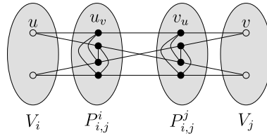
Fig. 1. An illustration of the gadget construction in the proof of Theorem 3.3.
