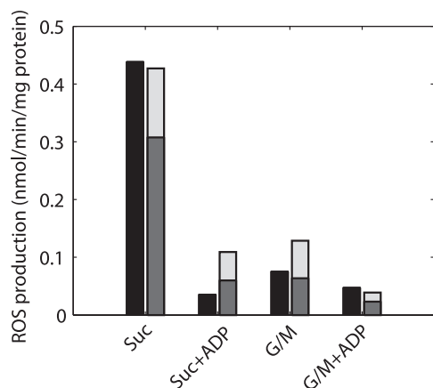
FIGURE 3 ROS production as a function of different substrates and mitochondrial respiratory states. Simulated state 4 ROS production in succinate ( Suc ; dark gray/light gray bar), predominated by RET-induced complex I ROS, quantitatively matches the experimental data (black). The bottom segment of each bar (dark gray) for the simulations depicts the ROS contribution from complex I, whereas the upper segment (light gray) depicts the contribution from complex III ROS production. During maximal rates of oxidative phosphorylation, stimulated by ADP (state 3), ROS production with succinate is minimized ( Suc+ADP ). ROS production with the complex I substrates ( G/M ) is split between complex I and complex III and is diminished when oxidative phosphorylation flux is maximal ( G/M+ADP ).
