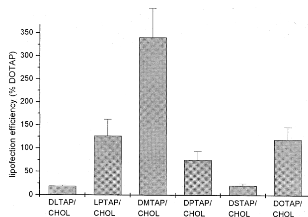
Fig. 5. Lipofection results of cholesterol-containing lipoplexes of DOTAP analogs (in a molar ratio of 1:2 of cholesterol:cationic lipid) and pCMXluc. Lipofection efficiencies (expressed in rlu/ \mu\text{g} of cellular protein) of the lipids were given as percentage of the DOTAP standard (set 100%). Experimental conditions were similar to other lipofection experiments (Figs. 3 and 4).
