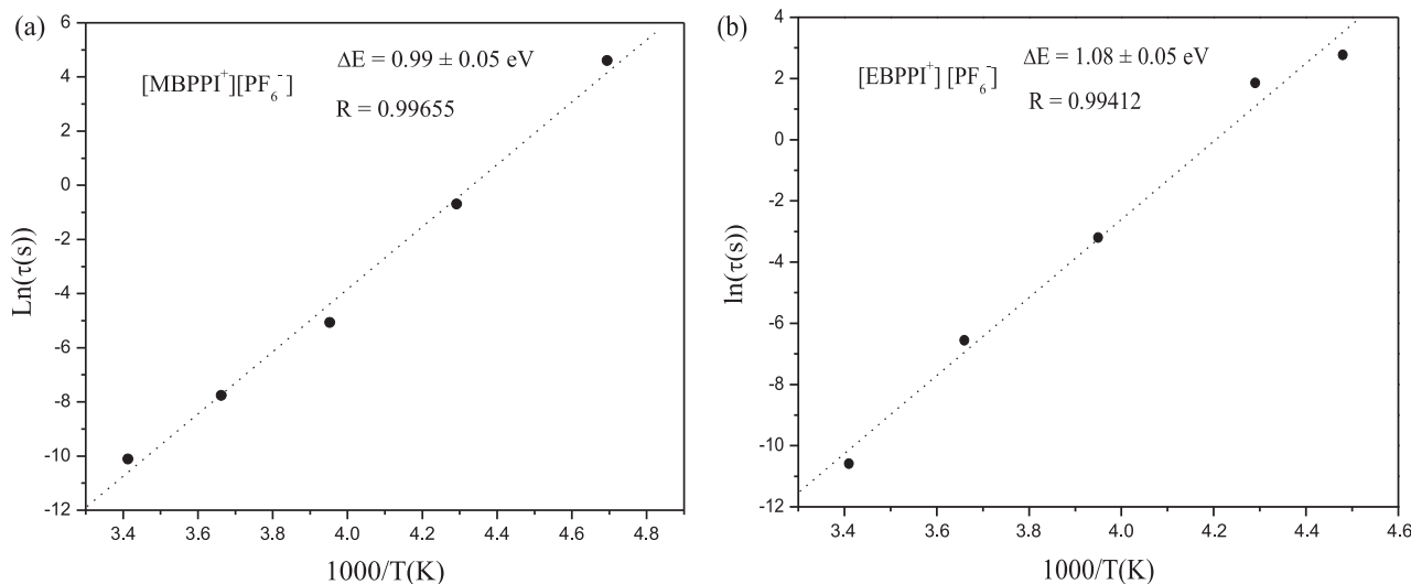
Figure 3 Temperature dependence of the relaxation times: Arrhenius plot of logarithm \text{Ln} \tau (●) vs. reciprocal of temperature 1/T . (····) Linear regression line. (R) correlation coefficient.
