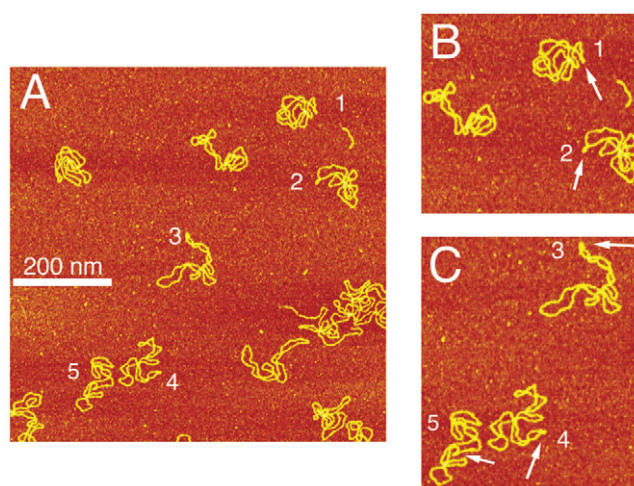
FIGURE 6 Atomic force microscopic images of pBan1 DNA. Large-scale scanning image is shown in panel A, and enlarged-rescanned images are shown in panels B and C. The molecules having the stem part at sharp turn region are numbered from 1 to 5.
