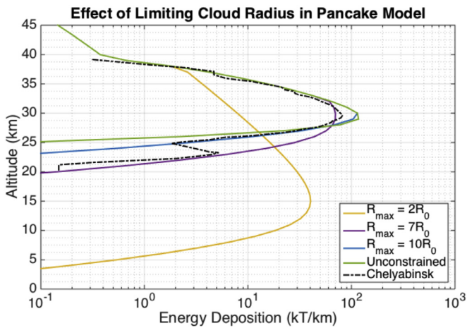
Fig. 8. Effects of cloud radius limits ( R_{max} ) on pancake model results for Chelyabinsk meteor energy deposition.
