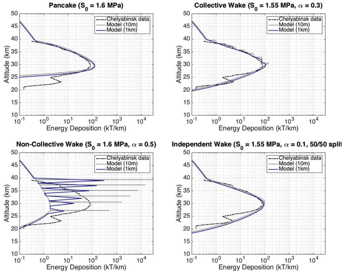
Fig. 6. Energy deposition curve from the pancake model and three discrete fragmentation models, matched to Chelyabinsk observational data with the parameters listed in Table 1.
