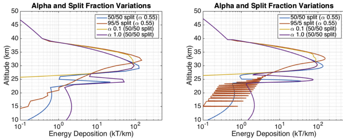
Fig. 10. Effects of different radius split fractions and \alpha values in the combination model, for the Chelyabinsk case with an initial breakup strength of 1.55 MPa (plotted at 1 km resolution on the left and 10 m resolution on the right).
