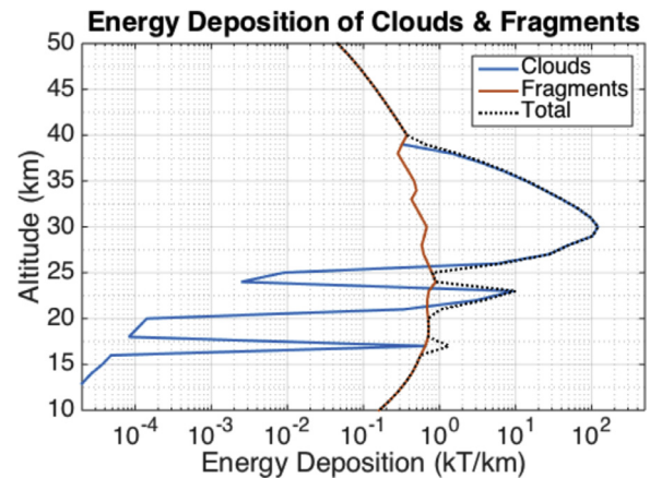
Fig. 9. Energy deposition contributions of the dust clouds and discrete fragments in the combination model. After initial fragmentation, the dust cloud dominates energy deposition, but later in flight the total is due mainly to the persisting fragments.
