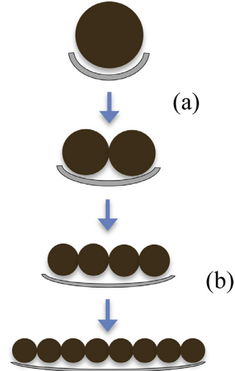
Fig. 2. Collective wake model. (a) Breaks and ballistic coefficient halves. (b) Process continues to ground under a single bow shock.
