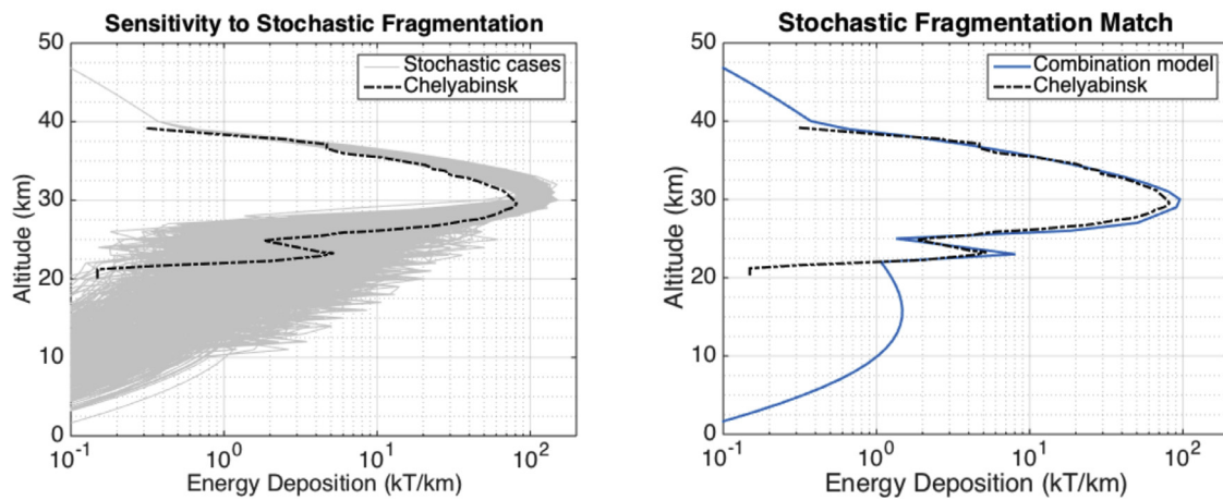
Fig. 11. Range of combination model results (left) and a sample curve-matched case (right) from 500 simulations of the Chelyabinsk entry case with strength scaling and radius split parameters varied stochastically at each fragmentation event: \sigma_0 = 1.55 MPa, \alpha = 0.1 –1.0, split fraction = 50/50–95/5 radius.
