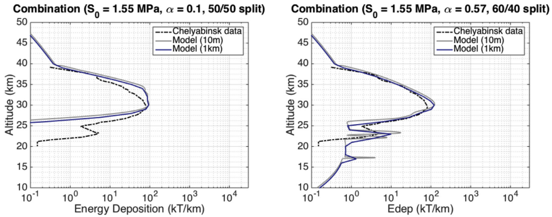
Fig. 7. Energy deposition curve from the combination model, matched to Chelyabinsk observational data with the parameters listed in Table 1.
