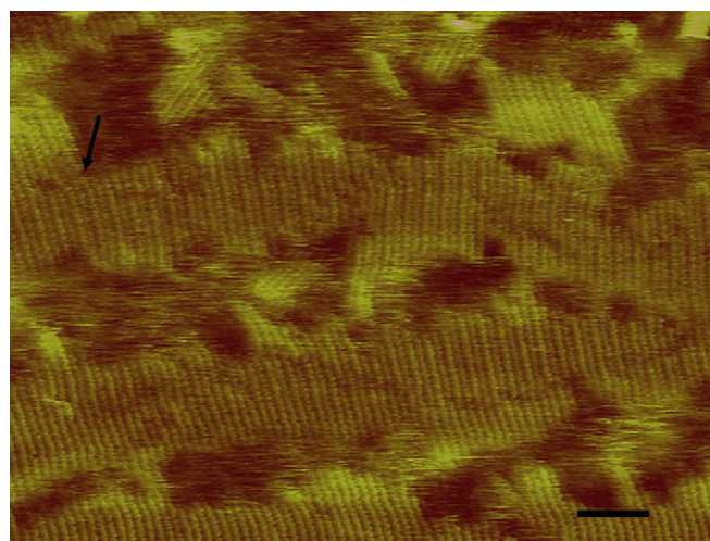
Fig. 9. An AFM topographic image of an it-PMMA Langmuir Blodgett film. The scale bar represents 10 nm. Reproduced from Ref. [85], with permission of ACS Publishing.
