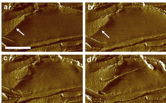
Fig. 7. A series of AFM phase images showing the formation of a screw dislocation branch in a polyethylene lamella. The arrow indicates the branch point. The scale bar represents 1 \mu\text{m} . Adapted from Ref. [58] and used with permission of Wiley-VCH.
