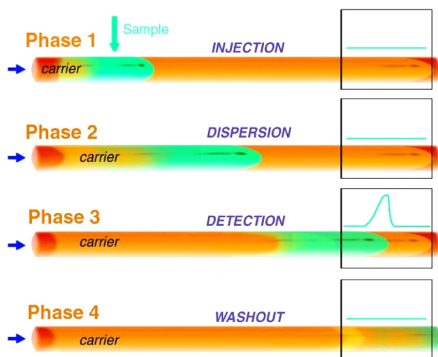
Figure 2 Stages of flow injection analysis. Source: http://ww2.chemistry.gatech.edu/class/analyt/fia.pdf .
