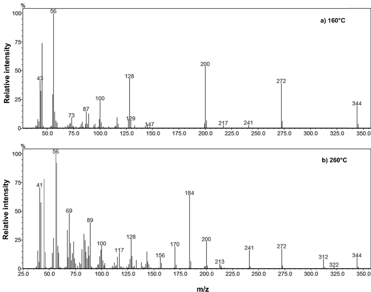
Fig. 2. Averaged mass spectrum for degradation products at 160 °C (a) and 260 °C (b) for the sample labelled 2.7HMIDI.
