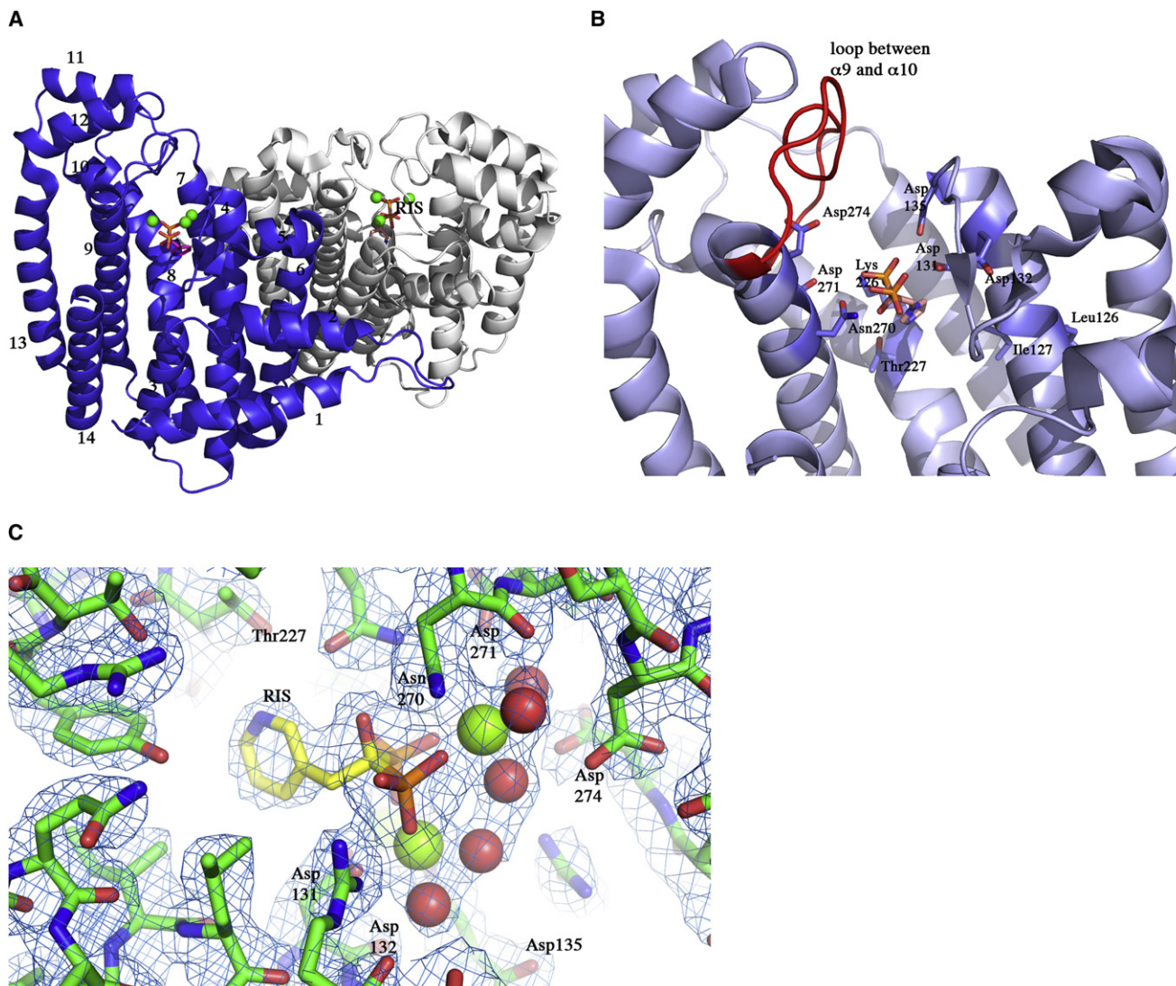
Figure 4. CpNPPPS Structures
