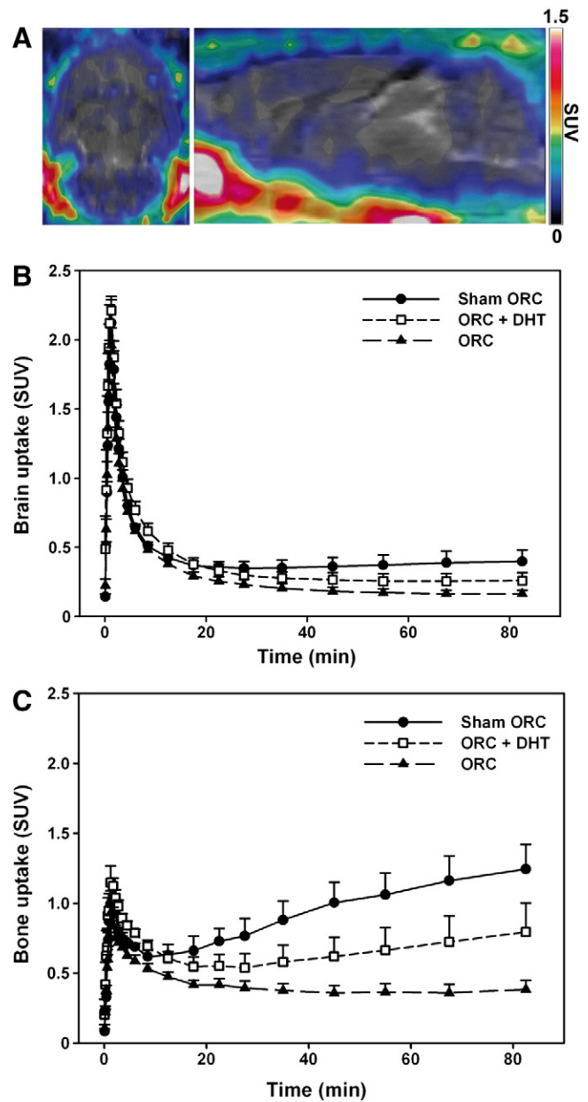
Fig. 2. (A) Representative coronal (left) and sagittal (right) [ 18 F]FDHT PET images of a rat brain. Images consist of the summed data from 50–90 min after tracer injection in a ORC rat. PET images are co-registered with an MRI template for anatomical reference. Time activity curves of [ 18 F]FDHT (standardized uptake value; mean \pm SEM) in the whole brain (B) and interparietal bone (C) in orchietomized rats (ORC, n = 6), orchietomized rats co-injected with 1 mg/kg dihydrotestosterone (ORC + DHT, n = 6) and sham-orchiectomized rats (Sham ORC, n = 5). No significant differences were observed in the time-activity curves in the whole brain. In contrast, [ 18 F]FDHT uptake in cranial bone was significantly higher in the distribution phase (3–90 min) in sham-orchiectomized rats than in orchietomized rats ( p < 0.05 ).
