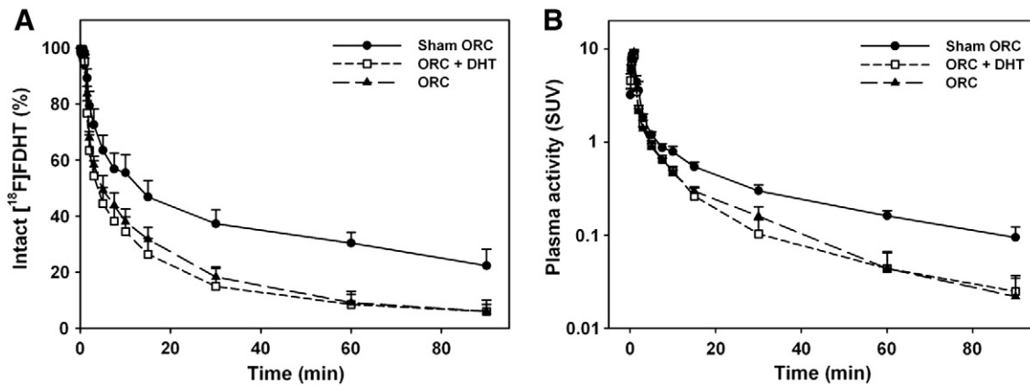
Fig. 3. (A) Percentage of intact [ ^{18}\text{F} ]FDHT in plasma and (B) metabolite-corrected plasma curves of [ ^{18}\text{F} ]FDHT in orchietomized rats (ORC, n = 5 ), orchietomized rats co-injected with 1 mg/kg DHT (ORC + DHT, n = 6 ) and sham-orchietomized rats (Sham ORC, n = 5 ) (mean \pm SEM). Sham-orchietomized rats showed a significantly higher percentage of intact tracer and metabolite-corrected plasma curve in the elimination phase of the time-activity curve (3–90 min, p < 0.05 ).
