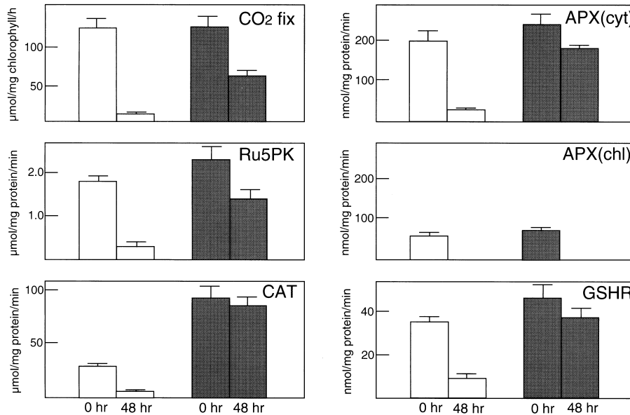
Fig. 5. Changes in activities of \text{CO}_2 fixation and enzymes after a shift from moderate light conditions ( 300 \mu\text{mol m}^{-2} \text{s}^{-1} ) at 60% relative humidity with periodic watering to drought conditions (60% relative humidity without watering for 48 h) at high light intensity ( 1600 \mu\text{mol m}^{-2} \text{s}^{-1} ). Total leaf activities of PRK, catalase (CAT) and GSHR were determined, as well as activities of cytosolic (cyt) and chloroplast (chl) isoforms of APX. The wild-type (open bars) and T43-1 (shaded bars) plants were analyzed before (0 h) and after (48 h) the stress treatment. Error bars show S.D.
