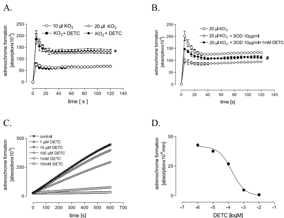
Fig. 3. Effect of 10 and 20 \mu l of a saturated KO_2 solution on formation of adrenochrome. A: DETC (1 mM) has no effect on adrenochrome formation. B: SOD inhibits adrenochrome formation by KO_2 and this effect is significantly reduced by the SOD inhibitor DETC (1 mM). C: Inhibitory effect of DETC on superoxide production by the X/XO system. D: Concentration-dependent inhibition of superoxide generation by DETC (* P < 0.001 for 10 \mu l KO_2 vs. 20 \mu l KO_2 , # P < 0.05 for KO_2 +SOD vs. KO_2 +SOD+DETC).
