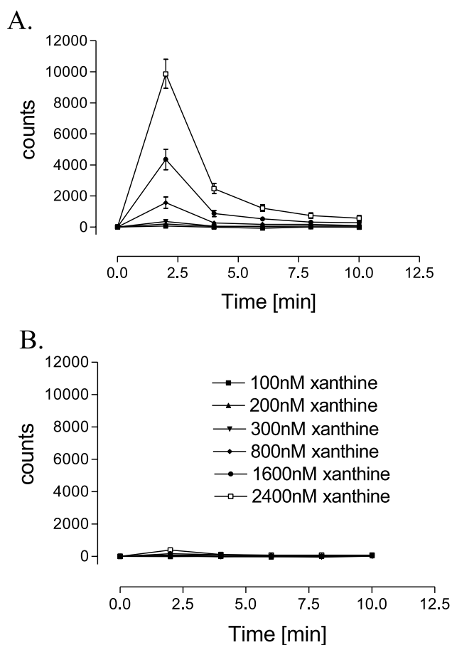
Fig. 2. Effect of 10 mM DETC on superoxide production by the X/XO system. A: Production of superoxide during incubation of XO with increasing concentrations of xanthine (0.1–2.4 \mu M). B: Production of superoxide during incubation of XO with increasing concentrations of xanthine (0.1–2.4 \mu M) in the presence of 10 mM DETC.
