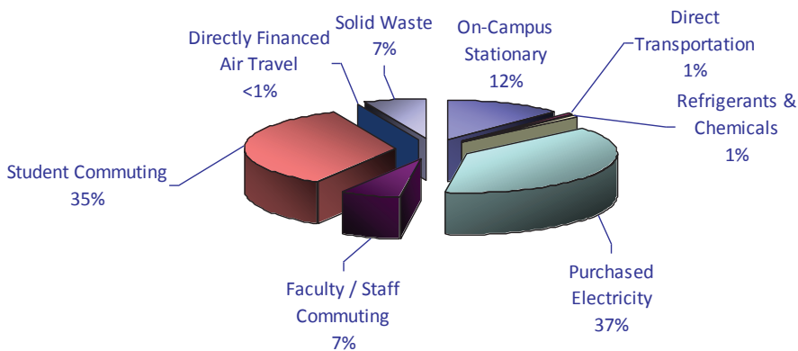
Figure 2: GHG Emissions by Sector – FY 2009
