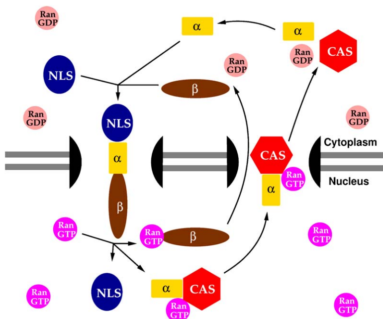
Figure 1. Schematic Diagram of the Primary Processes Involved in the CAS/Importin-β/α Nucleocytoplasmic Transport Cycle
