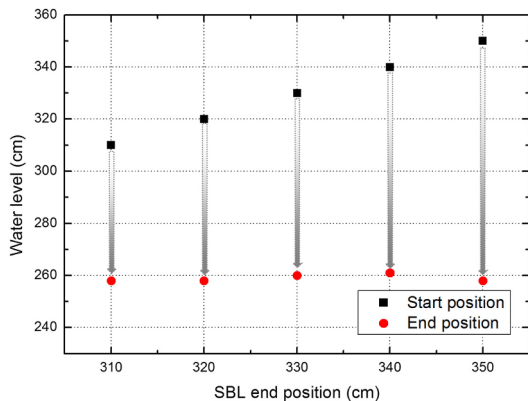
Fig. 5. Water Level Change during Siphon Breaking with Different Start Position of Siphon Break Line
