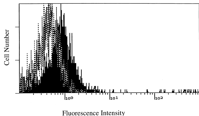
Fig. 3. Transfected WSL-1/TRAMP is expressed on the cell surface of HEK293T cells. 20 h following transfection of 6 \times 10^5 293T cells with 0.1 \mu\text{g} pCDNA3 WSL-1 expression construct the cells were harvested and stained with rabbit polyclonal anti-WSL-1/DR3 and the stained cells detected by flow cytometry (black histogram). Control untransfected cells were treated similarly (dotted histogram).
