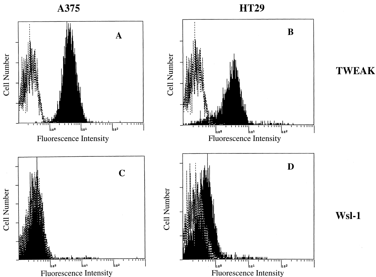
Fig. 4. Binding of TWEAK and WSL-1 to A375 and HT29 cells. Cells were incubated for 10 min in the presence (black histogram) or absence (dotted histogram) of 1 \mu\text{g} FLAG-tagged murine or human TWEAK (A and B). This was followed by a 10 min incubation with 0.5 \mu\text{g} anti-FLAG antibody and finally a 10 min incubation with 0.5 \mu\text{g} anti-mouse Alexa488. For WSL-1 binding (C and D) the cells were incubated for 10 min with 3 \mu\text{g} rabbit polyclonal anti-WSL-1/TRAMP antibody (black histogram). This was followed by a 10 min incubation with 0.5 \mu\text{g} anti-rabbit Alexa488. In all cases the cells were then washed in FACS buffer and analysed by flow cytometry. Control were treated in the same way, except that anti-WSL-1 was omitted (dotted histogram).
