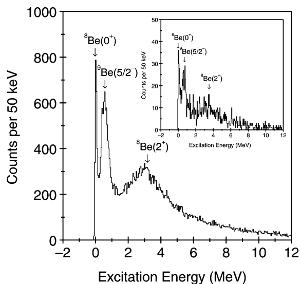
Fig. 2. The excitation energy spectrum corresponding to \alpha + \alpha coincidences from the ^{12}\text{Be} beam. The peaks correspond to the decay of the ground-state (92 keV) and the first excited state (3.04 MeV, 2^+ ). The peak at \sim 600 keV is produced by the decay of the 2.43 MeV ( 5/2^- ) state in ^9\text{Be} to the tail of the 2^+ state in ^8\text{Be} . The inset is the excitation energy spectrum corresponding to \alpha + \alpha coincidences from the ^{14}\text{Be} beam.
