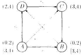
Fig. 5. An arc and path consistent form of the network in Fig. 4.
