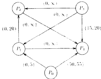
Fig. 24. The STP network of the singleton labeling of Fig. 23.
