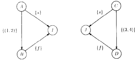
Fig. 25. A path consistent singleton labeling.
