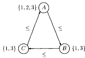
Fig. 13. An arc consistent CPA network over discrete domains.
