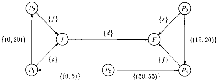
Fig. 23. A singleton labeling of the constraint graph of Fig. 2.
