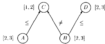
Fig. 22. A PA network over single-interval domains.
