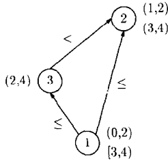
Fig. 16. A directional arc consistent form of the network in Fig. 11.
