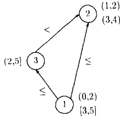
Fig. 11. The reduced network of the network in Fig. 4.
