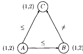
Fig. 19. The restricted network of the network in Fig. 18.
