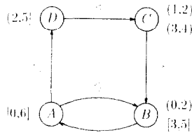
Fig. 4. A CPA network over multiple-intervals domains.
