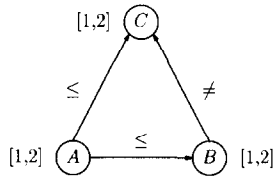
Fig. 18. An arc consistent PA network over single-interval domains.
