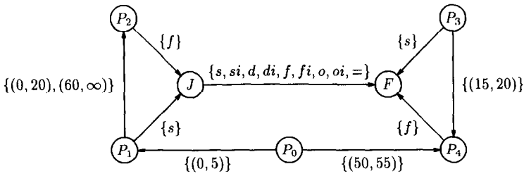
Fig. 2. The constraint graph of Example 2.1.
