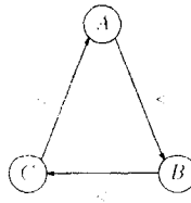
Fig. 17. An arc consistent CPA network.
