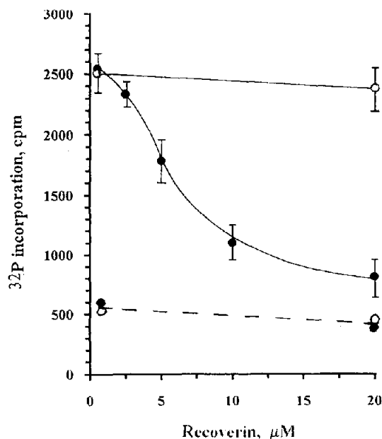
Fig. 2. Dependence of rhodopsin phosphorylation on recoverin concentration in the reconstituted system RK, urea-washed ROS membranes and recoverin. < 1 \text{ nM} and 5.6 \mu M free [Ca^{2+}] are referred to as 'low' ( \circ ) and 'high' ( \bullet ) [Ca^{2+}] , respectively. The reaction was carried out under light (solid line) or in the dark (dashed line). Points represent the average value ( n = 2 ) with S.D. bars.
