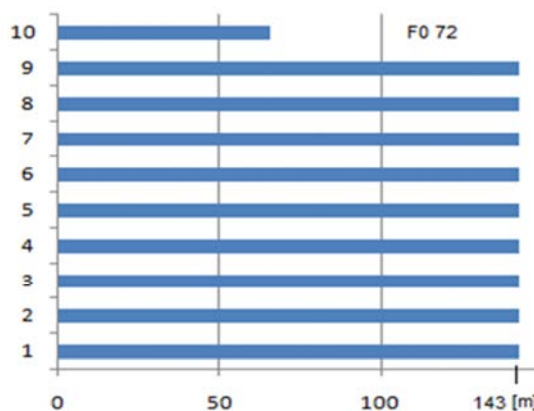
Fig.3. Maximum blowing distances for 10 optical fibers type Nexans, at 143 m distance, using a Microflow machine
