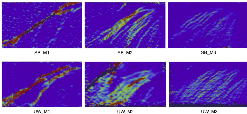
Fig. 14. Field of vertical axis deformations in the critical shear span of TRM-retrofitted specimens at the instant of peak load.
