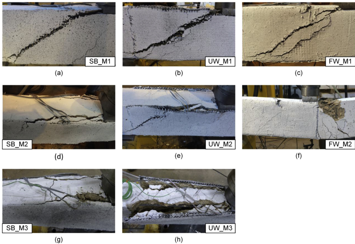
Fig. 9. Failure modes of TRM-retrofitted specimens: (a)–(c) Specimens SB_M1, UW_M1 and FW_M1 – local damage of the jacket; (d), (e) SB_M2 and UW_M2 – debonding of the jacket over a large area of the shear span: peeling off of the concrete cover; (f) FW_M2 – flexural failure despite the shear cracking of the TRM jacket; (g) SB_M3 – debonding of the jacket over a large area of the shear span: peeling off of the concrete cover; and (h) UW_M3 – abrupt debonding of the TRM jacket over the whole area of the shear span: peeling off of the concrete cover.
