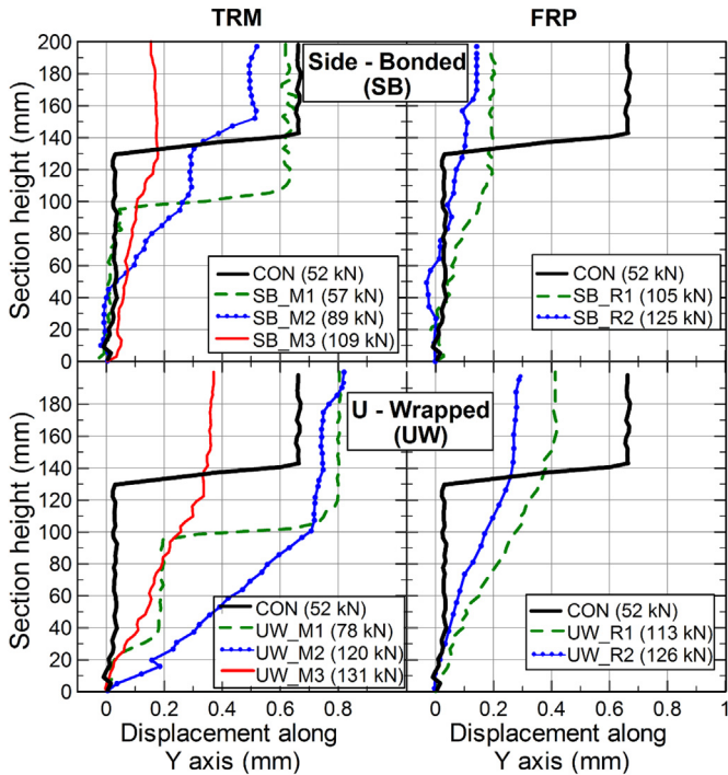
Fig. 13. Relative vertical displacements along the beam height at the central cross-section of the critical shear span, at the instant of peak load.
