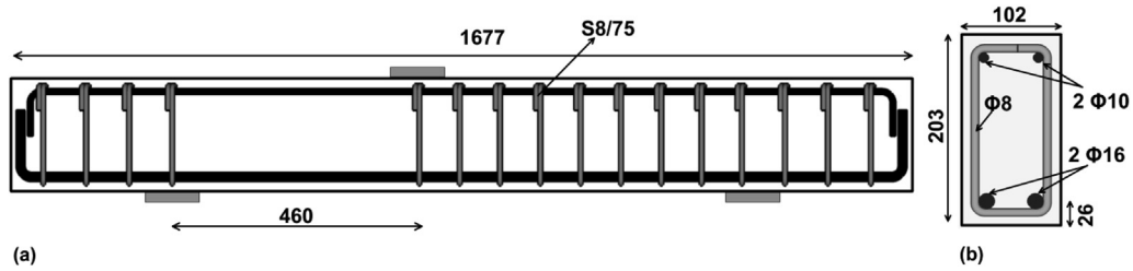
Fig. 2. (a) Beam geometry and reinforcement; (b) cross section (dimensions in mm).
