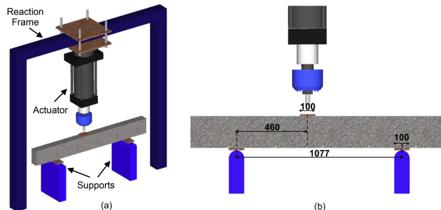
Fig. 1. Test set-up: (a) Overall 3D view; (b) front view.
