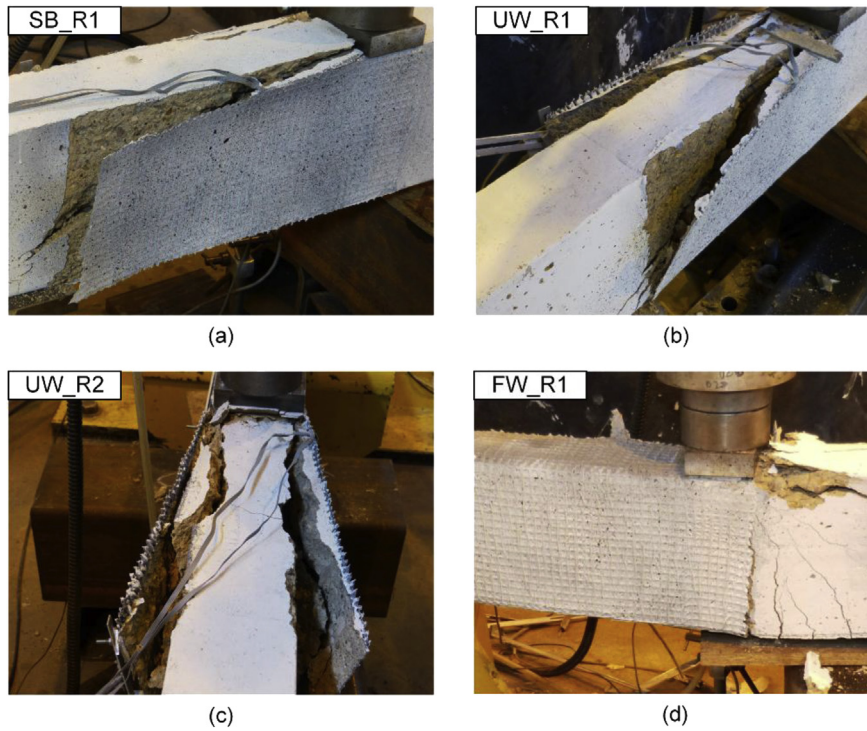
Fig. 8. (a) FRP debonding in SB strengthening configuration; (b), (c) FRP debonding in UW strengthening configuration; (d) flexural failure of specimen with FW FRP jacket.
