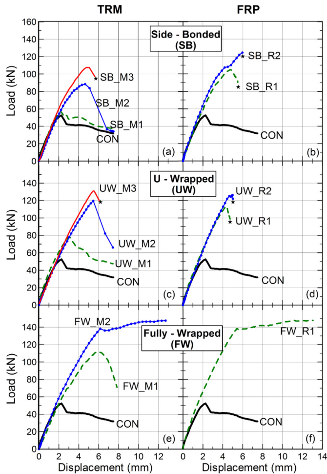
Fig. 6. Load versus vertical displacement curves for all tested specimens.
