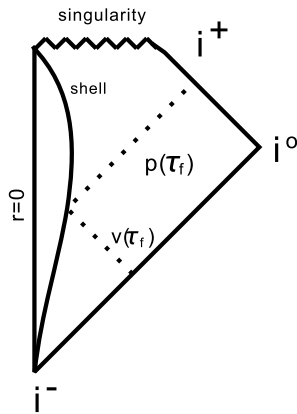
Fig. 3. Penrose diagram for the totally reflecting collapsing shell. The scalar field ingoing mode is reflected by the shell at time \tau_f .
