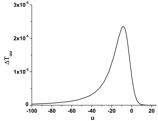
Fig. 5. The black curve represents the energy flux difference between totally reflecting shell and transparent shell, \Delta T_{uu} , at r \rightarrow \infty . At first, at u \rightarrow -\infty , there is no radiation and therefore no difference, so \Delta T_{uu} \rightarrow 0 . \Delta T_{uu} achieves its maximal at u \approx -8.3 . After that, radiation from both shells becomes very close to Hawking radiation, and \Delta T_{uu} goes back to zero.
