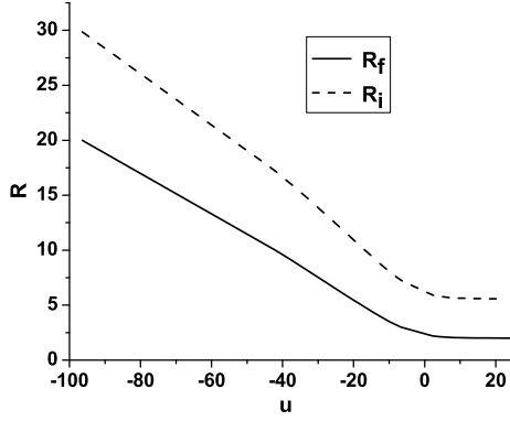
Fig. 2. In this figure we set u = t(\tau_f) - r^*(\tau_f) and M = 1 . R_i is the radius of the shell when the scalar field mode crosses it for the first time at \tau_i on the way inside the shell, and R_f is the radius when the mode crosses it for the second time on the way out \tau_f .
