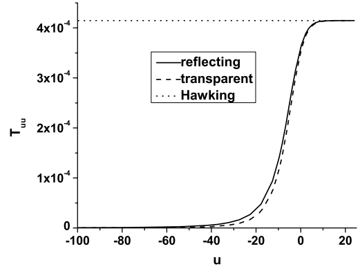
Fig. 4. The black curve represents the energy flux T_{uu} at r \rightarrow \infty for the totally reflecting shell. The dashed curve represents the energy flux T_{uu} at r \rightarrow \infty for the totally transparent shell. The dotted curve is the Hawking radiation for a static black hole, which is just \frac{1}{768\pi} . At late times, the two shells match the Hawking radiation from a pre-existing black hole, but the fluxes are substantially different during the collapse.
