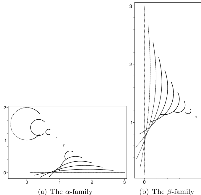
Fig. 3. Demoulin families of Dupin cyclides.
