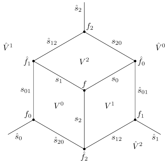
Fig. 2. A Bianchi cube.
