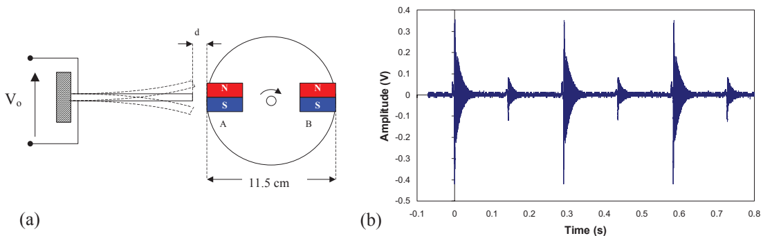
Fig. 9. Piezoelectric energy harevester from rotational motion based on impulse excitation: (a) structure; (b) and output voltage from the cantilever of Fig.1 for d = 2 mm at a rotating speed of about 3 rps.
