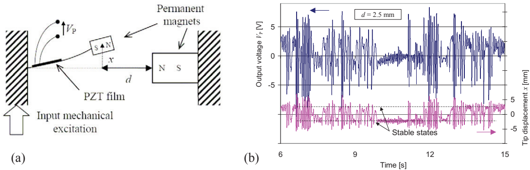
Fig. 8. Nonlinear piezoelectric energy harevester from vibration: (a) structure; (b) displacement and output voltage under bistable behaviour.
