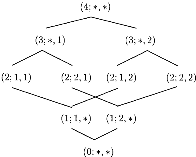
FIG. 1. P(3, \{[1, 2], [2, 3]\}, 2) .
