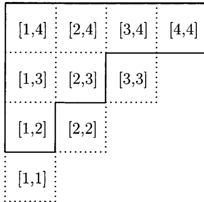
FIG. 2. Representation of the dual ideal \{[1, 2], [2, 3], [4, 4]\}^+ on [1, 4] .
