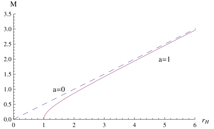
Fig. 1. It shows that the modification of relation between the event horizon and the mass. For a given mass M , the size of the classical black hole ( a = 0 ) is smaller than that of the quantum-corrected black hole ( a = 1 ), which can be seen clearly in the UV region.
