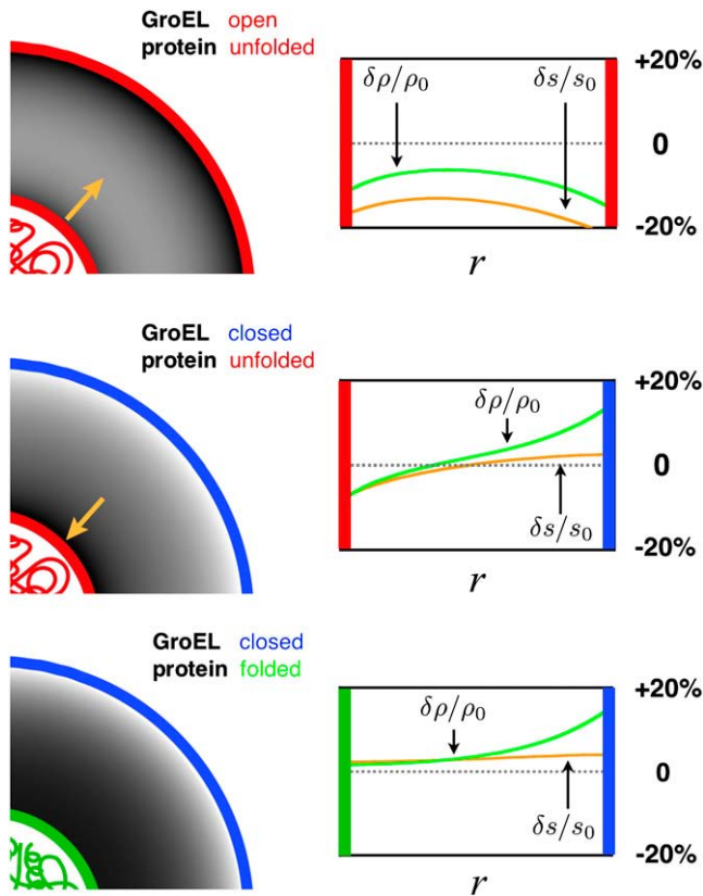
FIGURE 1 Equilibrium order parameters \delta\rho_{\text{eq}} and \delta s_{\text{eq}} inside spherical shells were calculated using m_\rho = 20 , m_s = 10 , D_\rho = 20 , D_s = 30 , \varepsilon = 5 , \rho_0 = s_0 = 1 , w = .5 , \bar{u} = 1 , R_p = 3 , and R_G = 7 . All data reported in this study use the same parameters for the free-energy functional. Units of length are set by \ell , the size of a water molecule ( \sim 4 \text{ \AA} ). Order parameters are unitless, and are measured as a fraction of their bulk value, whereas \varepsilon , m_\rho , and m_s have units of \text{kcal/mol}/\ell^3 , and D_\rho and D_s have units of \text{kcal/mol}/\ell . (Left) Liquid density (darker shading corresponding to lesser density) is plotted in the space between the surface of the protein (red, unfolded; green, folded) and the cavity (red, hydrophobic; blue, hydrophilic) wall for an unfolded protein inside an “open” hydrophobic cavity (top), an unfolded protein inside a “closed” hydrophilic cavity (middle), and a folded protein in a closed cavity (bottom). Gold arrows indicate the direction of solvent-mediated force between the two surfaces (Fig. 2) (Right) Liquid density (green curves) and hydrogen-bond order (orange curves) are plotted as a fraction of their bulk values. At a hydrophobic surface, there is a loss of hydrogen bonding and a depletion of liquid density. In contrast, at a highly hydrophilic surface, there is an elevation in liquid density and a greater amount of hydrogen bonding.
