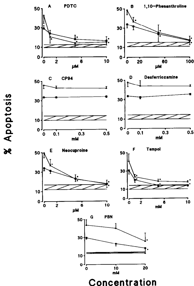
Fig. 1. Effects of free radical scavengers and metal chelators on dexamethasone and etoposide induced apoptosis. Thymocytes were incubated for 4 h with either dexamethasone (0.1 \mu\text{M} ) (■) or etoposide (10 \mu\text{M} ) ( \Delta ) and then apoptosis assessed by flow cytometry. Thymocytes were incubated in the presence of the indicated concentrations of various compounds and the results represent the mean \pm S.E.M. of at least three determinations. The shaded area represents the control level of apoptosis without any added inducing agent. *notes significantly different to the value obtained with either dexamethasone or etoposide alone, P < 0.05 .
