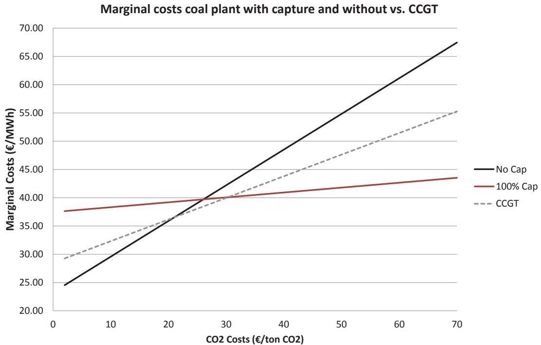
fig. 5 Marginal Costs of a coal plant with and without capture vs. CCGT plant
