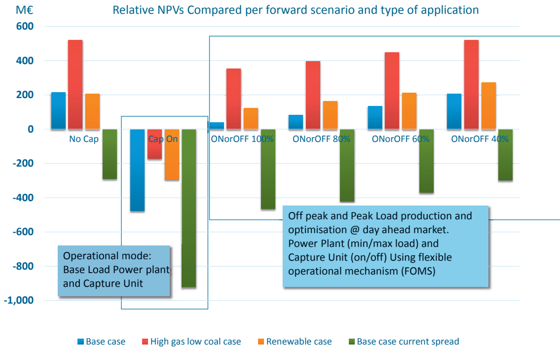
fig. 7 Relative NPV analysis at different forward price scenarios and capture size.
