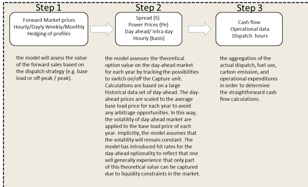
fig. 2 Methodology buildup of the plant value
