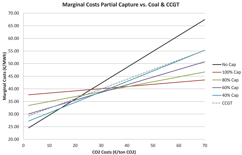
fig. 6 Marginal costs different size capture units
