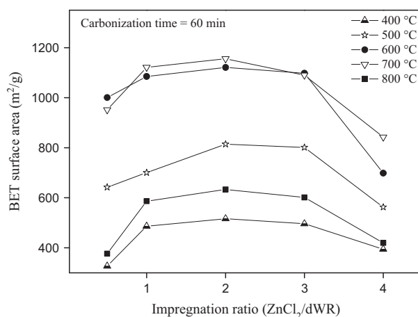
Figure 1 Influences of carbonization temperature and impregnation ratio on the surface area of prepared WACs.
