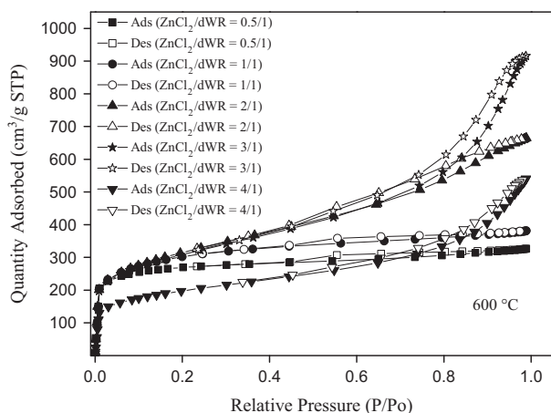
Figure 3 N_2 adsorption–desorption isotherms of WACs prepared for different impregnation ratios ( ZnCl_2/dWR ) at 600 °C.
