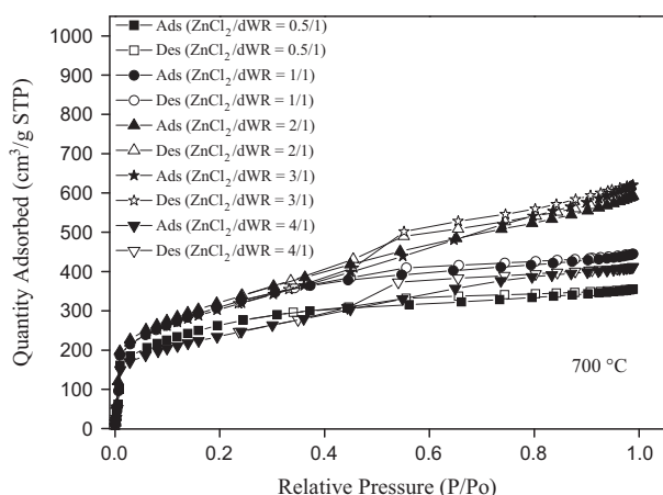
Figure 4 N_2 adsorption–desorption isotherms of WACs prepared for different impregnation ratios ( ZnCl_2/dWR ) at 700 °C.
