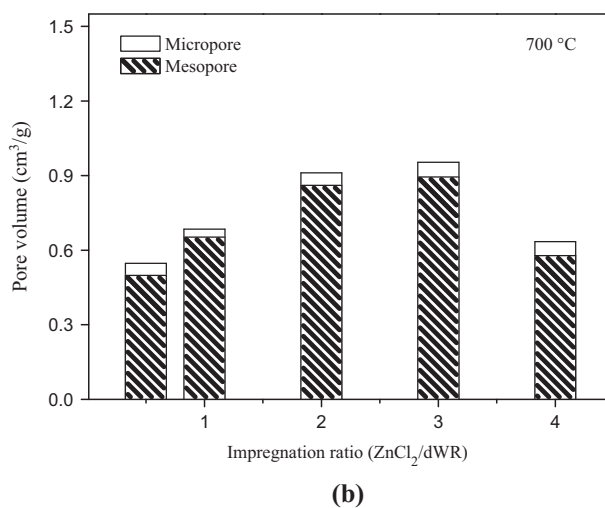
Figure 2 Influences of impregnation ratio on the micropore and mesopore volumes of prepared WACs at (a) 600 and (b) 700 °C.
