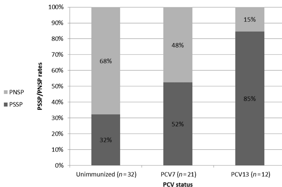
Figure 1. PNSP/PSSP partition in Sp positive MEF cultures from “severe” AOM episodes, according to PCV status. The overall PNSP rate was 51% (31% intermediate, 20% resistant) and demonstrated statistically significant association on PCV-status ( p = 0.006 ). Unimmunized children had higher PNSP rate than PCV7 immunized children ( p = 0.15 ), and higher PNSP rate than PCV13 immunized children ( p = 0.002 ). AOM = acute otitis media; MEF = middle ear fluid; PCV = pneumococcal conjugate vaccine; PCV7 = 7-valent pneumococcal conjugate vaccine; PCV13 = 13-valent pneumococcal conjugate vaccine; PNSP = Penicillin nonsusceptible Streptococcus pneumoniae ; PSSP = Penicillin susceptible Streptococcus pneumoniae ; Sp = Streptococcus pneumoniae .
