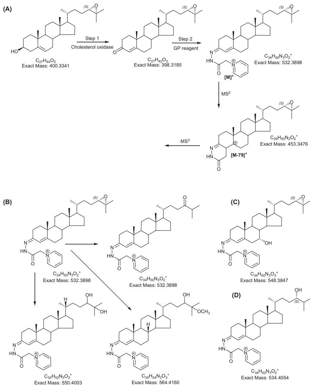
Fig. 1. (A) Oxidation with cholesterol oxidase (step 1), followed by derivatisation with the GP reagent (step 2) and fragmentation by mass spectrometry ( MS^2 ). The reactions are exemplified by 24S,25-epoxycholesterol. (B) Structure of 24S,25-epoxycholesterol its isomer 24-oxocholesterol and hydrolysis and methanolysis products after oxidation/derivatisation. (C) Structure of 3 \beta ,7 \alpha -dihydroxycholesterol-5-en-24S,25-epoxide and (D) 24S-hydroxycholesterol following oxidation/derivatisation.
