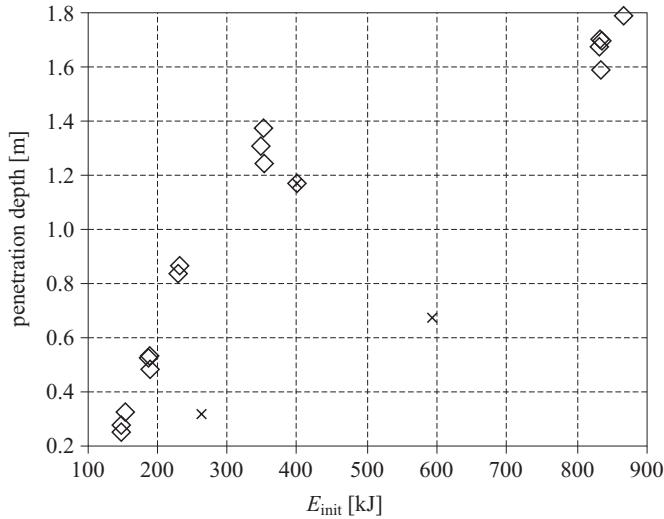
Figure 11. Predicted bubble penetration depth as a function of the initial wave packet energy, according to the formula given by Chanson & Lee (1997). The symbols ( \times ) and ( \diamond ) refer to spilling and plunging waves respectively
