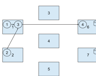
Fig. 5. Deployment 1
