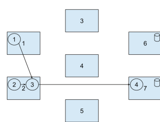
Fig. 6. Deployment 2
